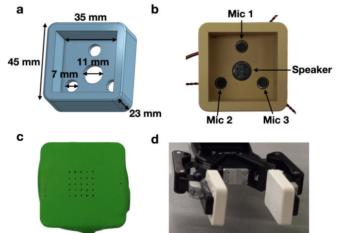
Fig. 2: Planar tactile sensor design. (a) CAD drawing with dimensions. (b) Location of speaker and microphones. (c) Rubber membrane interface for tactile sensing marked with a 5 \times 5 grid to evaluate contact location estimation. (d) Planar sensor attached to robotic gripper arm.
