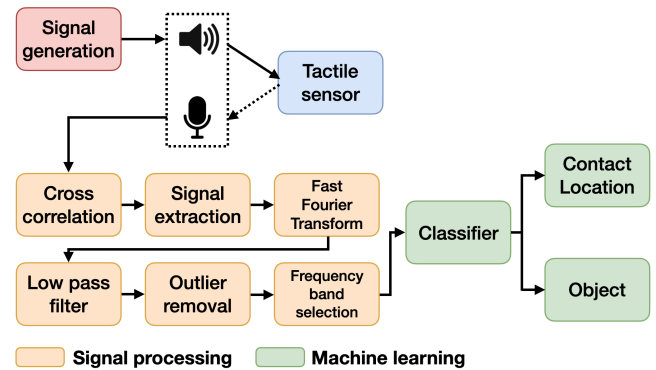
Fig. 3: Tactile sensing pipeline for contact point estimation and object classification.
