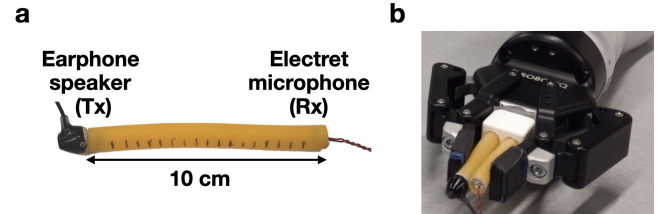
Fig. 1: Linear tactile sensor design. (a) Speaker and microphone are coupled to opposing ends of the rubber tube. Surface markings used for contact location estimation evaluations are separated by 5 mm. (b) Linear tactile sensor attached to existing robotic gripper arm (Robotiq 2F-85 gripper end-effector [1]) to enable sensing of different objects.
