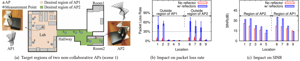
Figure 8: Experiments on efficacy of reflectors confining wireless coverage and reducing interference. (a) shows the placement and desired Wi-Fi regions of two APs. (b) plots the packet loss rate change outside the desired region of each AP when optimized reflectors are placed. (c) presents reflectors' impact on SINR inside the AP's desired region.
