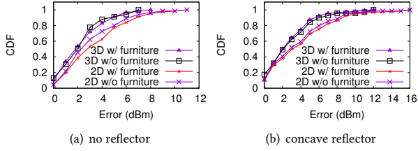
Figure 10: Accuracy of 3D wireless propagation modeling, in comparison to the 2D modeling in prior work [16].
