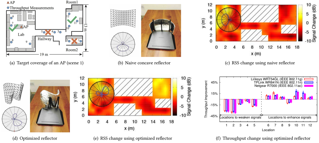
Figure 6: Efficacy of an optimized reflector for achieving a target wireless coverage (a), where areas users aim to strengthen the signal are marked by green ticks and areas to weaken the signal are marked by red crosses. (b) and (c) show a reflector in a simple concave shape and its resulting signal change in dB, while (d), (e), and (f) show a reflector in optimized shape, and the resulting changes in signal distribution and throughput. The optimized reflector shape leads to a signal distribution better matching the target.
