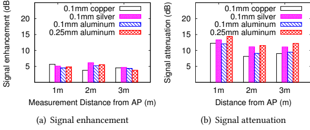
Figure 5: Different plane reflector’s ability to reflect and attenuate Wi-Fi signals, at distances from 1 to 3 meters.
