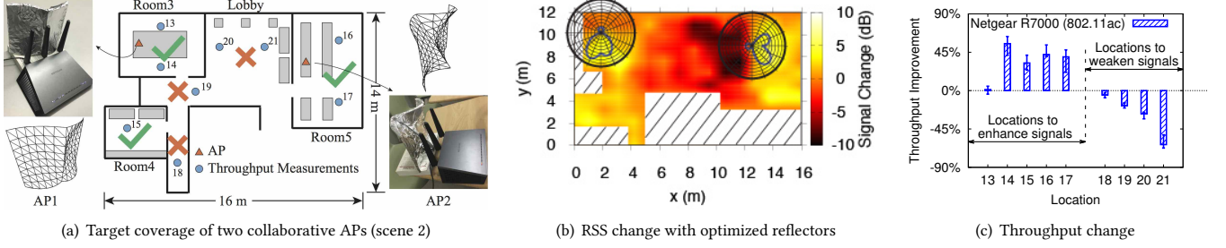
Figure 7: Efficacy of optimized reflectors of two collaborative APs to achieve a target wireless coverage. In (a), areas where users aim to strengthen or weaken signals are marked by green ticks and red crosses, respectively. (b) shows the map of resulting signal change in dB. (c) plots the throughput improvement at sampled locations (blue circles in (a)).
